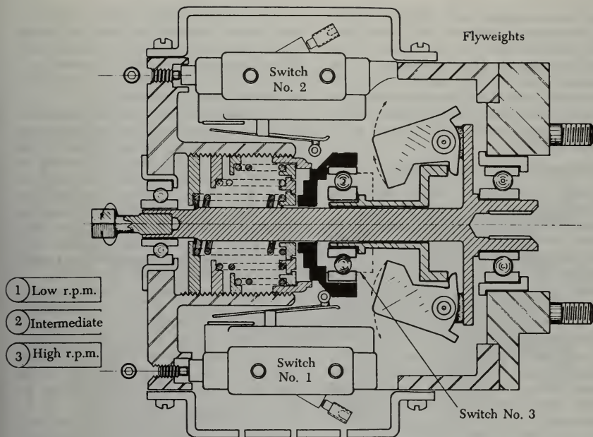
FIGURE 3-45. Speed-sensitive control.
